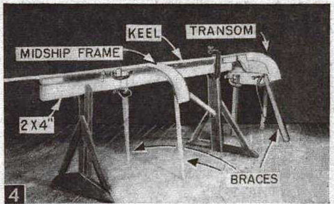
4 Midship frame and transom are kept in alignment with braces toe-nailed to the floor and clamped to the frame parts.
