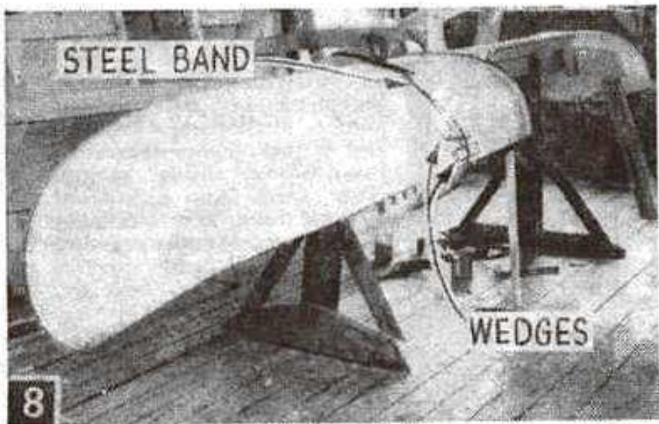
One sheet of 4 x 8 ft. plywood planks forward half of the canoe.
