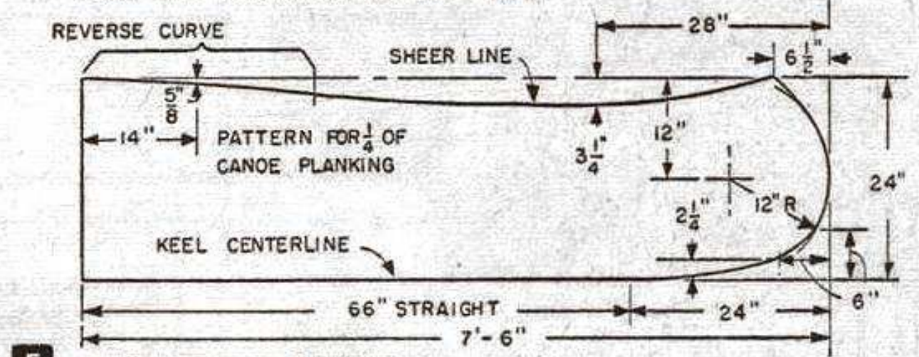
5 PLANKING PATTERN & LAYOUT
